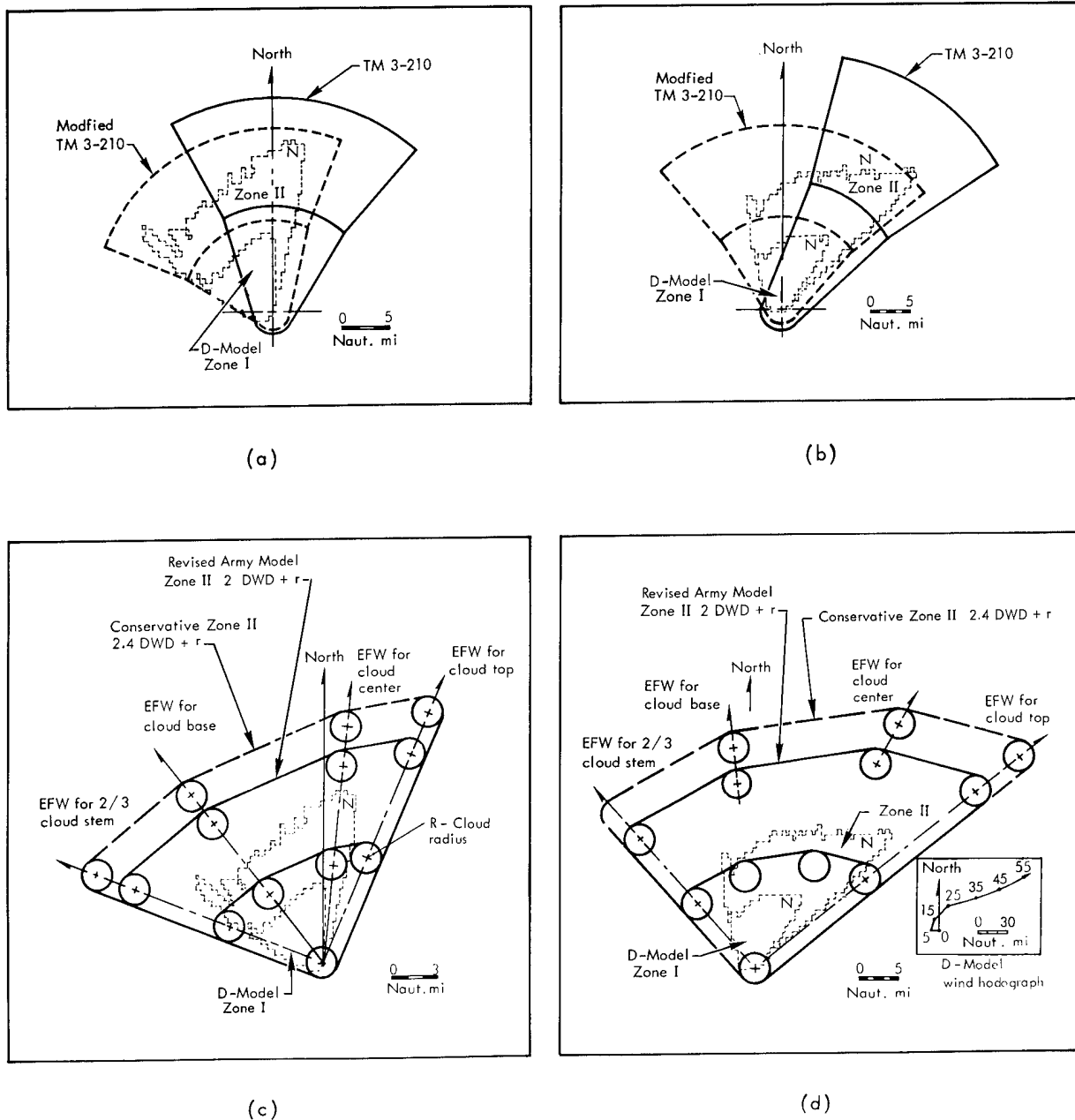
Fig. 13. NRDL modifications to a) the Army model for 10 kt, and b) the Army model for 50 kt. Characteristics of the D-Model are added to the Army model in c) for 10 kt and in d) for 50 kt. (From Ref. 23.)
